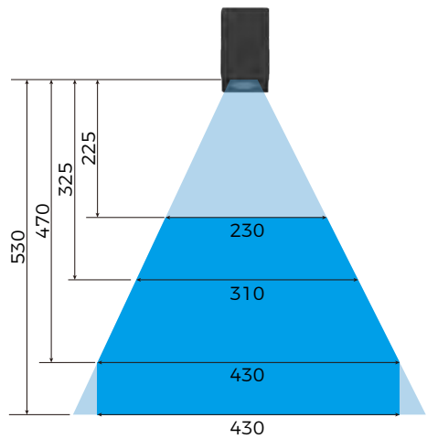
Mech-Eye LNX-8300
